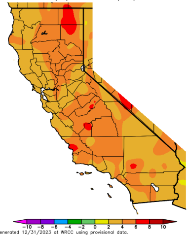
Fig 1: December 1st – December 30th Temperature Departure from Average Percent of Average Precipitation (%) 12/1/2023 – 12/30/2023
