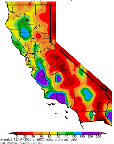
Fig 2: December 1st – December 30th Precipitation (% of Ave.)
