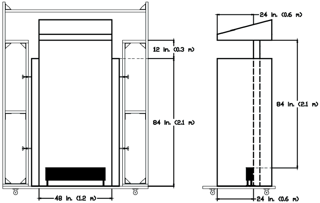
FIGURE 12-7A-3-1. EAVES-WALL TEST ASSEMBLY
